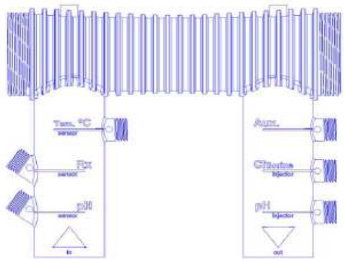
Vista frontal
